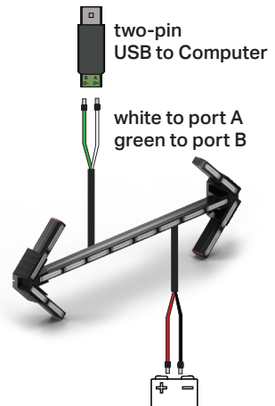
two-pin wiring harness connects usb to computer
