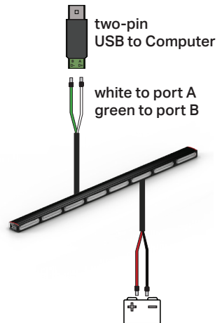
two-pin wiring harness connects usb to computer
